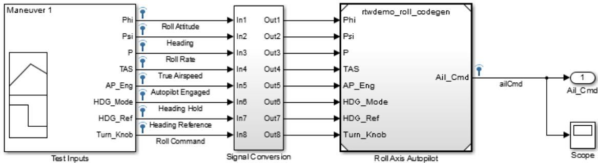
Test Harness For Roll Axis Autopilot Model
